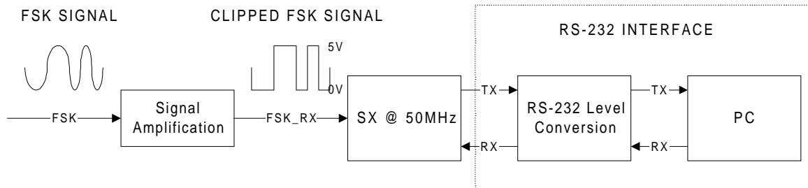
Figure 3-1. Hardware for FSK Demodulation
