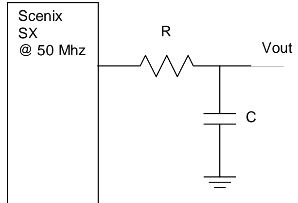
Figure 5-1. Circuit Diagram
